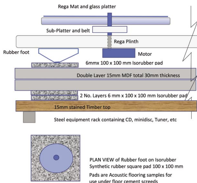
A fine diagram supplied by Ron Koorm of his turntable isolation system for a Rega RP3 turntable. "You don't have to spend a small fortune on special isolating plinths" he says.
